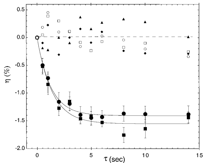
FIGURE 3 Truncated driven ^{19}\text{F}\{-^1\text{H}\} NOE selected in the backbone amide proton region at 8.79 ppm ( \square , \blacksquare , \blacklozenge ) and the indole N-H proton region at 10.03 ppm ( \circ , \bullet , \blacktriangle ) to ^{19}\text{F} in F3 ( \square , \blacksquare , \circ , \bullet ) or F6 ( \blacklozenge , \blacktriangle ). Open and filled symbols are measurements in the absence and presence of gramicidin, respectively. With 400 \mu\text{M} gramicidin A, \langle\Sigma\sigma\rangle between F3 and the backbone and indole amide protons was 0.0105 \pm 0.0014 ( n = 8 ) and 0.0106 \pm 0.0007 ( n = 12 ), respectively. Solid lines are best fit to the data using Eq. 1. The dashed line is a visual guide indicating no NOE build-up in either F3 in the absence of gramicidin or in F6 in the presence of gramicidin. Error bars show the standard error of the mean.
